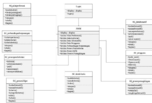
Gambar 4. Class Diagram
