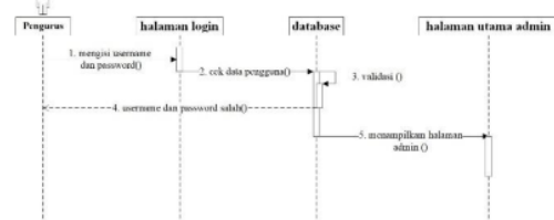
Gambar 2. Sequence Diagram Login
